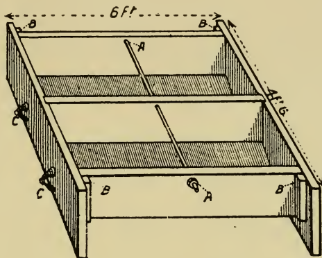
Fig. 76.—HONEY TANK. (Not drawn to scale.)
