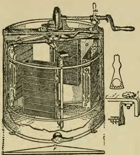
Fig. 43.—“ AUTOMATIC ” FOUR-COMB REVERSIBLE EXTRACTOR.
