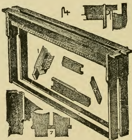
Fig. 32.—THE HOFFMAN BROOD AND EXTRACTING FRAMES.
