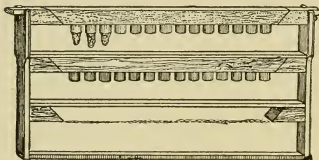
Fig. 53.—CELL-BASES SPIKED TO THE BARS OF A FRAME.
