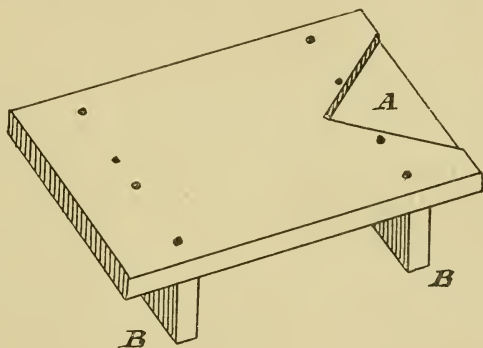
Fig. 24.—BOTTOM BOARD.
