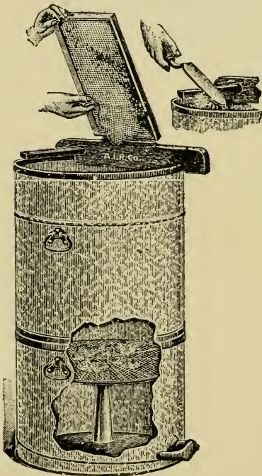
“DADANT” UNCAPPING CAN.
