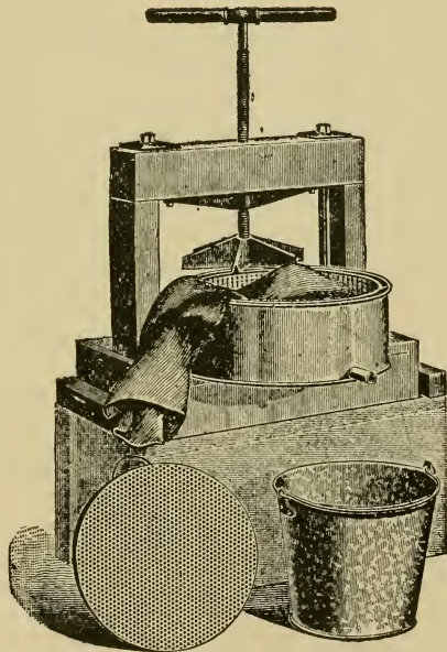
Fig. 13.—"HATCH" WAX PRESS.
