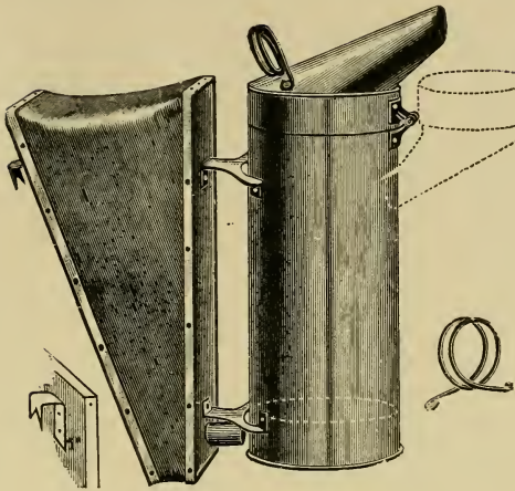
Fig. 48.—CORNEIL SMOKER.
