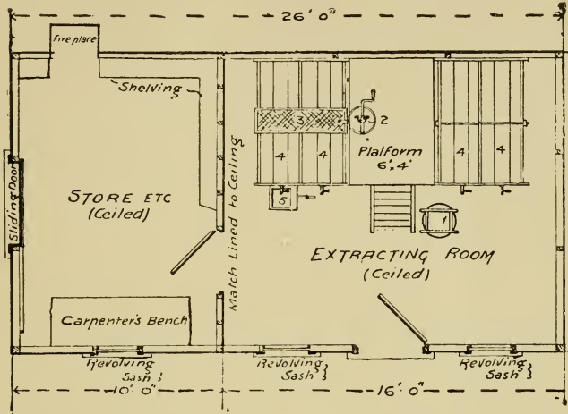
Fig. 17.—GROUND PLAN OF EXTRACTING HOUSE AND HONEY STORE ROOM.
